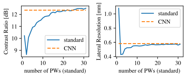
Fig. 2. Contrast ratio and lateral resolution reached by our CNN model with 3 PWs ( -15^\circ, 0^\circ, +15^\circ ), compared to the standard compounding of m PWs spanning uniformly a \pm 15^\circ sector (uniform scheme). Contrast ratio is measured on a B-mode image (gamma-compression, \gamma = 0.3 ) using an anechoic region, while lateral resolution is measured on the envelope image of 0.1mm nylon fibers. Both measures were obtained from data acquired from the Gammex phantom.
