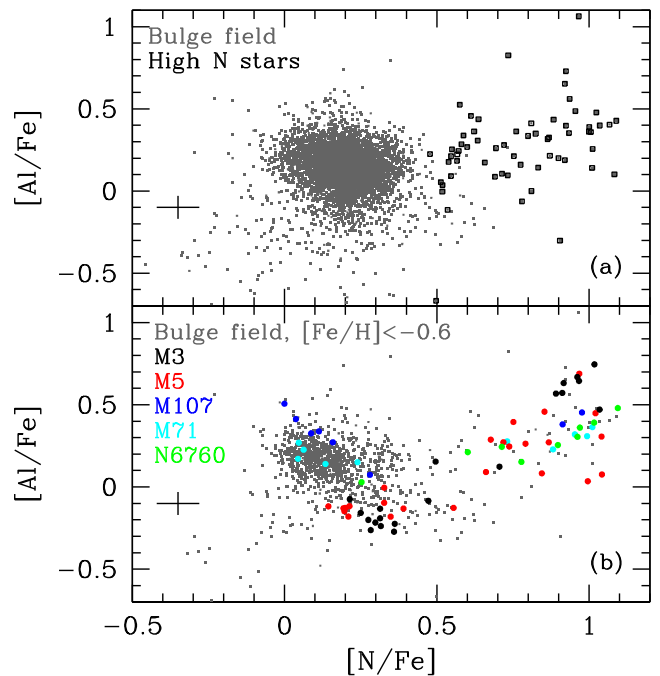
Figure 3. Sample stars in another chemical abundance diagnostic plot, adopting same symbols as in Figs 2(a) and (b). (a) A correlation between [\text{N}/\text{Fe}] and [\text{Al}/\text{Fe}] is evident in the N-rich sample (squares), whereas an anticorrelation appears to be present for stars with normal nitrogen abundances ( [\text{N}/\text{Fe}] \lesssim +0.5 ). (b) The SG stars in GCs, with [\text{N}/\text{Fe}] \gtrsim +0.5 , occupy the same locus as the N-rich population, following a similar correlation between the two abundance ratios. On the other hand, FG stars in GCs follow the same trend as the lower [\text{N}/\text{Fe}] field stars. This plot corroborates the notion that the N-rich stars inhabit the same region of chemical composition space as SG stars from GCs. The GC sample has few counterparts to the field stars with intermediate nitrogen ( 0.5 \lesssim [\text{N}/\text{Fe}] \lesssim 0.7 ) in panel (a). It is unclear whether this is a real effect or whether it is due to limitations in the APOGEE GC sample, which is relatively small.
