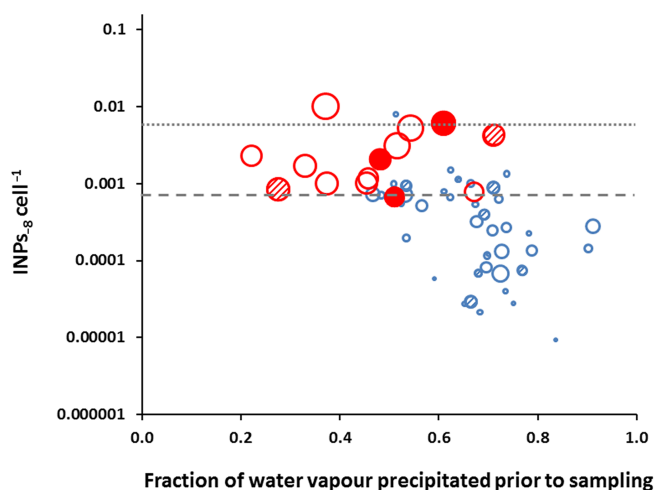
Figure 3. Ratio of INPs 8 to bacterial cells in precipitation samples collected at Jungfraujoch (3580 m a.s.l.). The width of symbols is proportional to wind speed (minimum = 2 km h -1 , maximum = 89 km h -1 ). Red symbols correspond to values with average wind speeds > 50 km h -1 during samplings, and blue symbols correspond to data with lower wind speeds. Patterned symbols represent the 10 samples in which P. syringae was searched for but not found. The three full symbols represent samples where culturable P. syringae was found. Dashed and dotted lines indicate median and maximum ratios observed in cloud water collected over the course of a year at Puy de Dôme (1465 m a.s.l.), 350 km west of Jungfraujoch (data from Joly et al., 2014).
