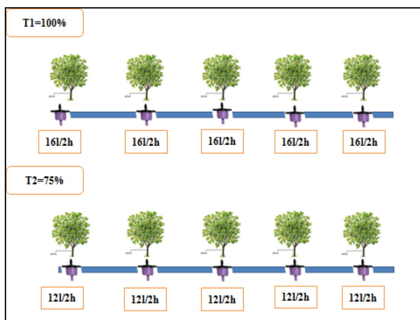
Figure 1: Illustration of the experimental device on the peach orchard
