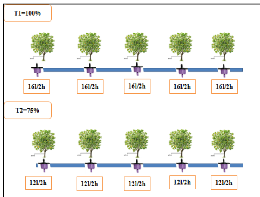
Figure 1: Illustration of the experimental device on the peach orchard
