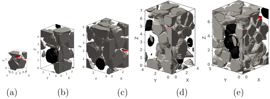
Fig. 2. Several sub-volumes cut in the whole voxel-based microstructural model: (a) 0.5M.STRUCT; (b) 5M.STRUCT; (c) 9M.STRUCT; (d) 17M.STRUCT and (e) 30M.STRUCT. Units on the axes are in mm.
