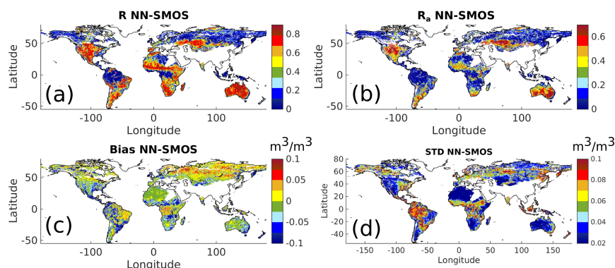
Figure 6. Comparison of AMSR-E NN SM and SMOS L3 SM from June 2010–October 2011. (a) Local Pearson correlation of the two SM datasets; (b) local Pearson correlation of the anomalies of the two SM datasets; (c) bias (mean AMSR-E NN SM minus mean SMOS L3 SM); (d) standard deviation of the difference of the two SM datasets.
