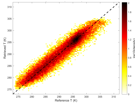
Figure 3. Scatter plot of the soil temperature retrieved with the neural network using T_b^H at 23 GHz and both T_b^H and T_b^V at 36 GHz (Model 7 in Table 2) versus ERA-Land soil temperature in the first layer (0–7 cm). The scatter plot is represented as the density of points in a logarithmic scale.
