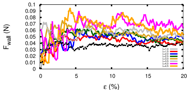
Fig. 7. A Compressive force on the top wall as a function of vertical deformation \varepsilon = \delta h/2R for all value of size ratio \lambda .
