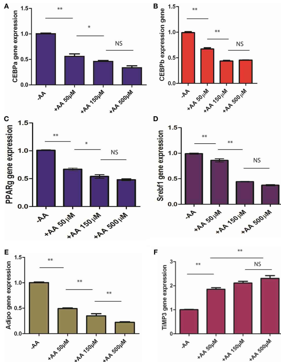
FIGURE 3 | Markers expression. 3T3 L1 were cultured without IBMX and without or with different concentrations of AA. RNAs were extracted after 9 days and expression of different genes, CEBPα (A), CEBPβ (B), PPARγ (C),
