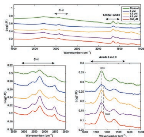
► Figure 3: (Top) sFTIR raw spectra in the 4,000\text{--}1,000 \text{ cm}^{-1} region recorded at a single-cell scale on E. coli grown without (control) or in the presence of ionic silver at lethal ( 100 \mu\text{M AgNO}_3 ) or sub-lethal ( 5.0, 6.5, 8.5 \mu\text{M AgNO}_3 ) concentrations. The regions of interest are identified by horizontal arrows in the figure; (Bottom left) Focus on the fatty acid region ( 3,050\text{--}2,800 \text{ cm}^{-1} ); (Bottom right) Focus on the peptide region ( 1,800\text{--}1,300 \text{ cm}^{-1} ), including amide I and amide II bands, which are characteristics of the peptidic bonds of peptides and proteins. The downshift in the amide I band ( \alpha -helix, 1650 \text{ cm}^{-1} ) between control E. coli cells (in green) and 100\text{-}\mu\text{M AgNO}_3 treated cells (in red) is also indicated as an example.
