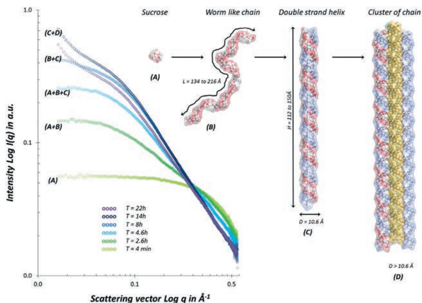
► Figure 2: SAXS curves of amylose synthesized by NpAS at different reaction times. Model of amylose chains in wormlike structure, double helix and packing of double helices leading to crystallization.
