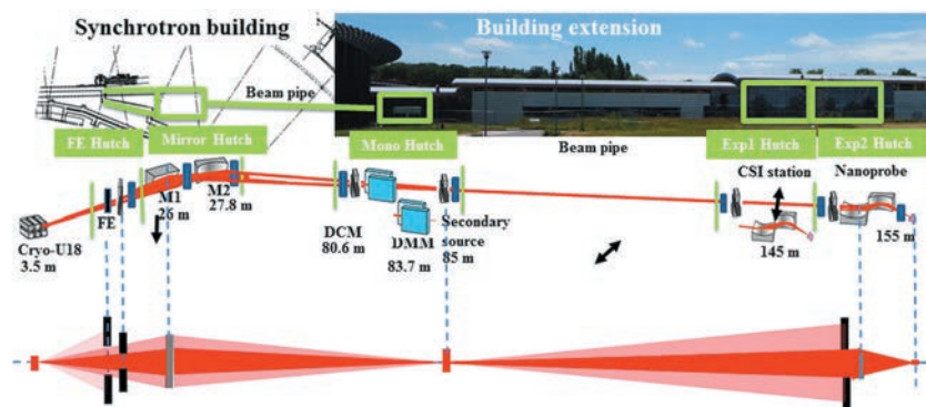
► Figure 2: General layout of the Nanoscopium beamline.
