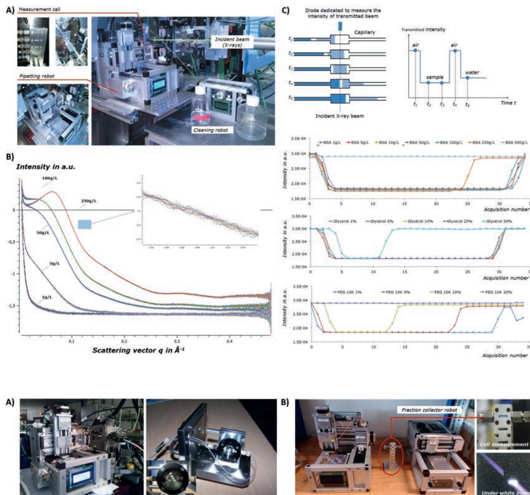
► Figure 2: A) The pipetting robot installed on SWING beamline to perform SAXS experiments. B) SAXS curves obtained with a set of BSA concentrations. For each concentration, 20 injections and measurements were performed and superimposed. C) Evaluation of the ability of the robot to manipulate viscous solution. The transmitted X-ray beam through the capillary is measured with a diode. For each solution and concentration, an intensity profile is plotted to follow the progression of the sample through the capillary.
