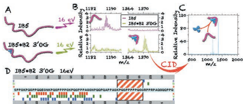
► Figure 2: Localization of the B2 3'OG binding site on IB5. The objects IB5 + and IB5•B2 3'OG + were selected and irradiated with 16 eV photons (A). Comparison between the MS/MS 16 eV VUV spectra identified specific fragments in the IB5•B2 3'OG + fragmentation spectrum in which the m/z ratio had a mass difference corresponding to that of B2 3'OG + , and fragments from the fragmentation spectrum of IB5 + (B). CID activation of identified fragments confirmed the presence of the ligand (C). The map of B2 3'OG-carrying fragments identified the 'KPQGPPPPQGG' sequence as a B2 3'OG binding site on IB5 (D).
