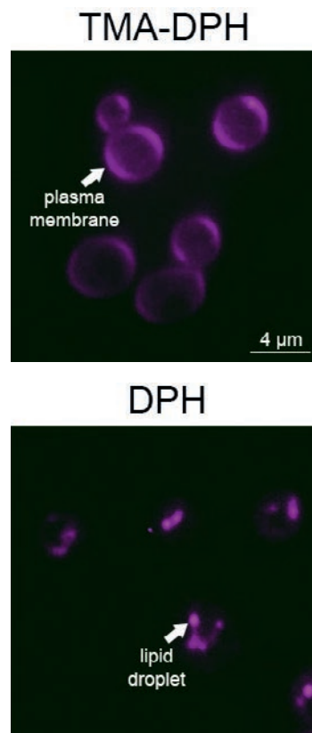
► Figure 2: Saccharomyces cerevisiae cells stained with TMA-DPH (top) or DPH (low). TMA-DPH is mainly associated with plasma membrane and DPH with round intracellular structures corresponding to lipid droplets.
