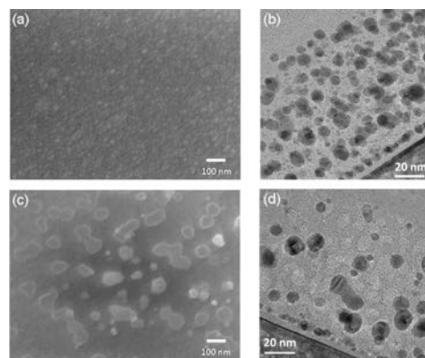
► Figure 2: SEM planar views (a,c) and TEM micrographs (b,d) of the plasma-deposited nanosilver-coating; (a,b) before ageing; (c,d) after ageing in saline solution ( \text{NaCl } 150 \text{ mM} ).
