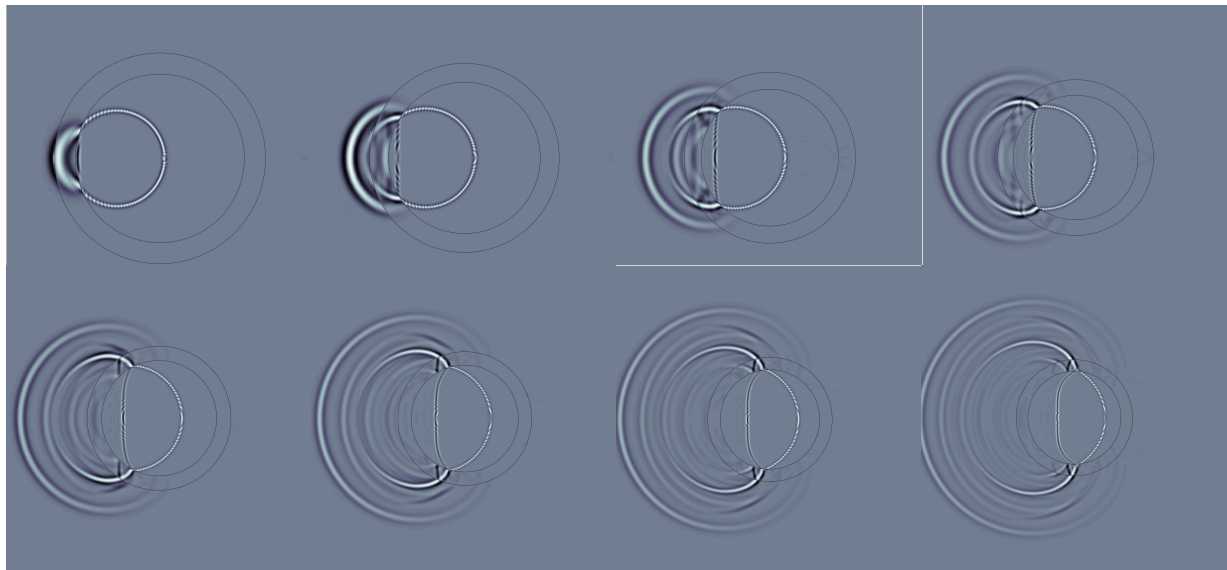
Figure 3. Pressure and radial stress resulted from an internal incident pressure P-wave, for different time values.
