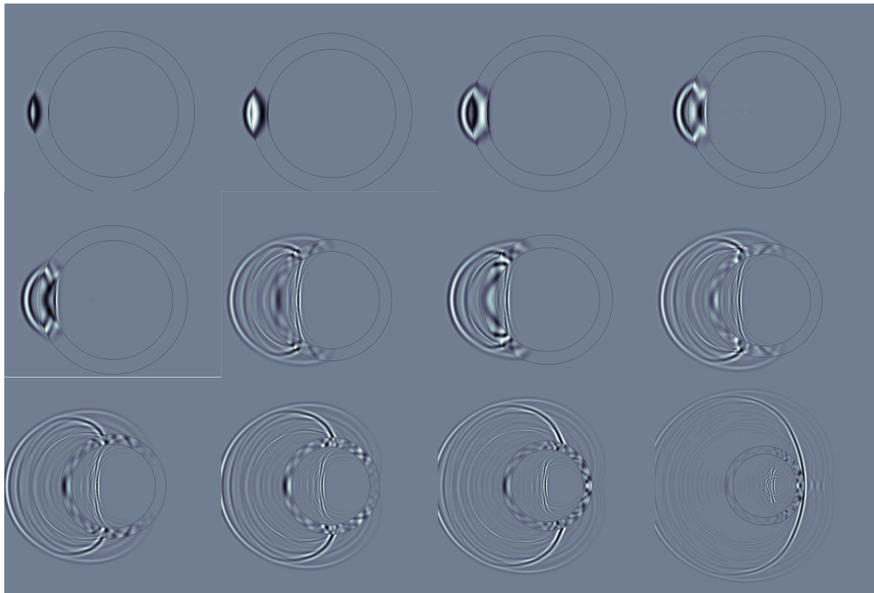
Figure 2. Pressure and radial stress resulted from an elastic, incident P-wave coming from a point located in the external elastic medium, for different time values.
