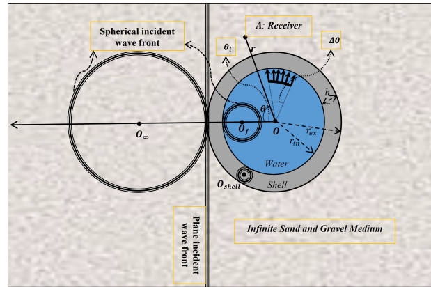
Figure 1. The problem's geometry
