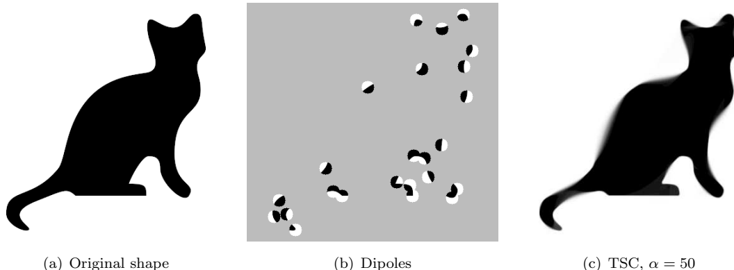
Figure 7: Computation of “Weickert’s cat” [67]: (a) shows the original shape, (b) depicts the given dipole data and (c) is the result of minimizing the TSC energy in the gray inpainting domain.
