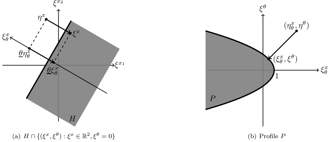
Figure 3: Projection of the point (\eta^x, \eta^\theta) onto the convex sets H . First, the point (\eta^x, \eta^\theta) is projected onto the profile P which yields (\xi_\theta^x, \xi^\theta) , then \xi^x is computed from \xi_\theta^x via the geometric relationship \xi^x = \eta^x - \underline{\theta}(\eta_\theta^x - \xi_\theta^x) .
