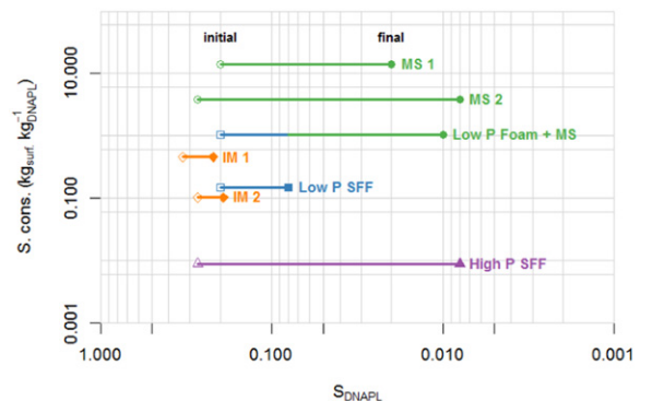
Fig. 6. Remediation technology performances.
