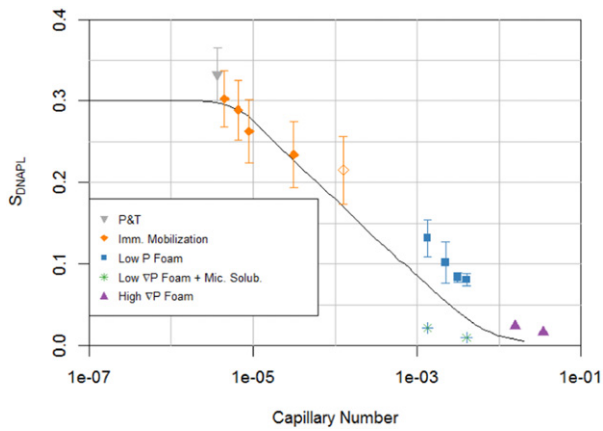
Fig. 7. S_{DNAPL} vs. N_{Ca} for mobilization experiments using water alone, surfactant solution, low and high \nabla P foams and low \nabla P foam completed by micellar solubilization. Curve is theoretical data from (Lake, 1989).
