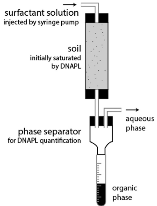
Fig. 1. Experimental set-up.
