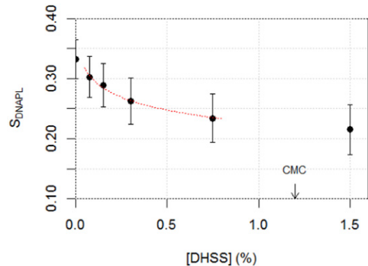
Fig. 4. Equilibrium DNAPL saturation after flushing with different surfactant concentrations. Dotted line is logarithmic fit of experimental data.
