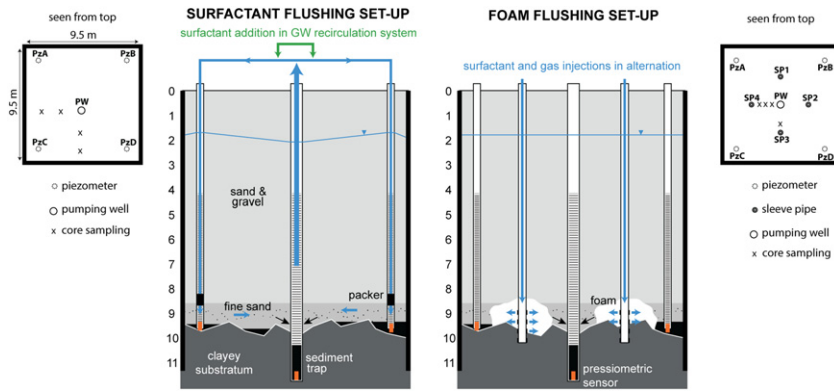
Fig. 2. Field set-up for surfactant flushing with GW recirculation and SF flushing.
