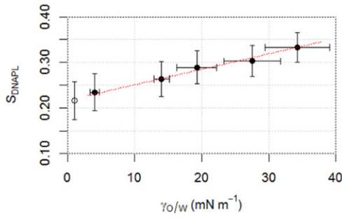
Fig. 5. Relationship between \gamma_{ow} and equilibrium DNAPL saturation.
