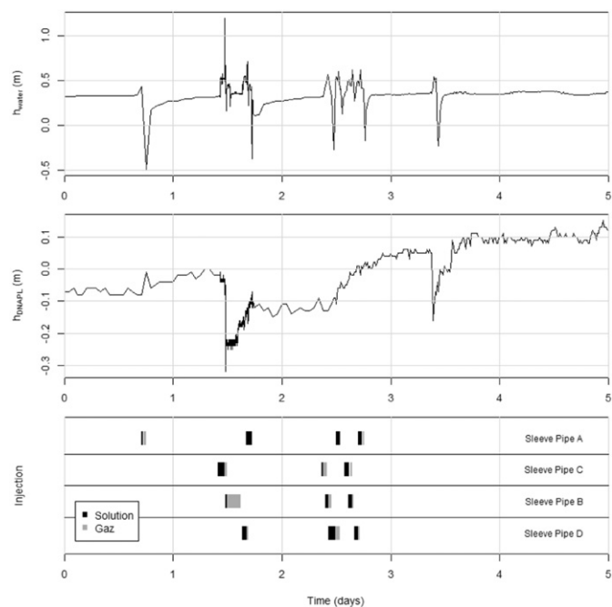
Fig. 9. Variation of the water table level and DNAPL interface level in the recovery well during the foam injection test. The spike during day 3 is due to water injection for pipes cleaning.
