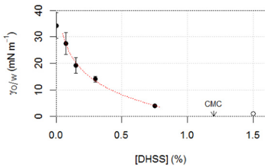
Fig. 3. Variations of \gamma_{ow} with DHSS concentration in lab-tests. The dotted line is the logarithmic fit of experimental data. \gamma_{ow} could not be measured accurately for [DHSS] = 1.5%.
