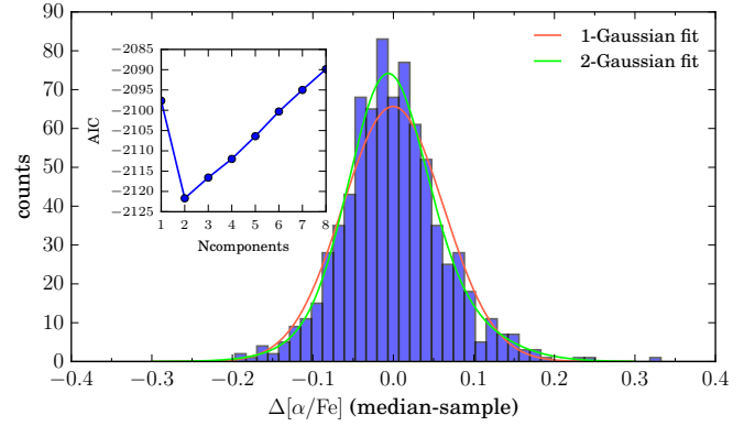
Fig. 1. Gaussian mixture method analysis of the [\alpha/\text{Fe}] abundance distribution with respect to the median values along the sequence. The inner panel shows the Akaike information criterion for different numbers of components. The best fit (green curve) corresponds to the two-component mixture. The red curve shows the poorer quality fit of the single Gaussian component, whose probability of explaining the distribution is 21 times lower than the double Gaussian component.
