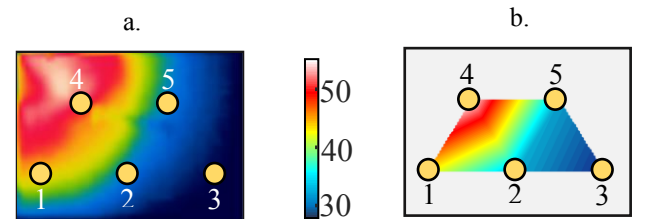
Fig. 2. Temperature field (in °C) on the composite plate obtained with the thermal camera (a.) and estimated using the static capacity measurements (b.)
