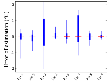
Fig. 4. Error of temperature estimation for the 8 healthy PZTs obtained on 54 random measurements between 15 and 21 °C.
