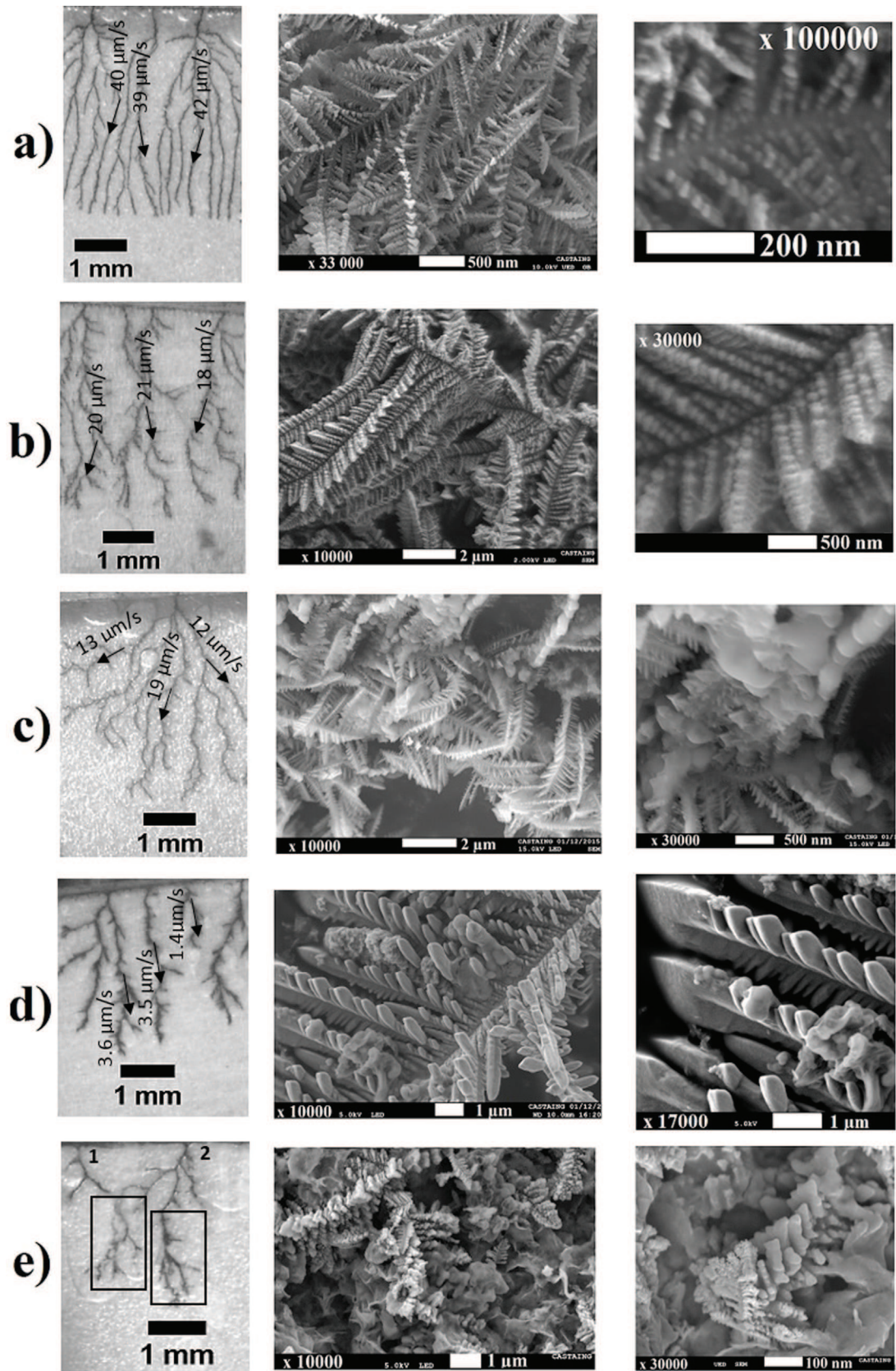
Fig. 7. SEM pictures of iron electrodeposits obtained in the Hele-Shaw cell at various current densities and using various precursor concentrations. a), b), c) 0.02 M \text{FeCl}_2 using 24, 12 and 8 \text{mA/cm}^2 respectively; d), e): 0.1 M \text{FeCl}_2 using 12 and 8 \text{mA/cm}^2 respectively. Millimetric (left column), micrometric (middle column) and nanometric (right column) scales. Some values of the growth velocity are indicated on the left pictures.
