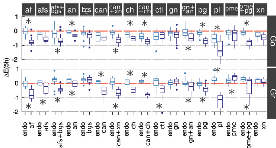
Fig. 2. Effects of endogenous (endo) and exogenous enzymes on the storage modulus of Golden Delicious (Go) and Granny Smith (Gr) apple varieties after 5 h incubation in the reaction medium. Enzyme codes are given in Table 1. * Significantly different ( P < 0.05 ). Cellulase (can and ctl), pectin methylesterase (pme), and \alpha -fucosidase (afs) did not affect the modulus of Go parenchyma tissue. Xyloglucanase (xn) did not modify the modulus of Gr. \beta -galactosidase (bgs) did not affect either Go or Gr. All other enzymes and combinations significantly affected the mechanical properties of the cortex parenchyma tissue in both Go and Gr. (This figure is available in colour at JXB online.)
