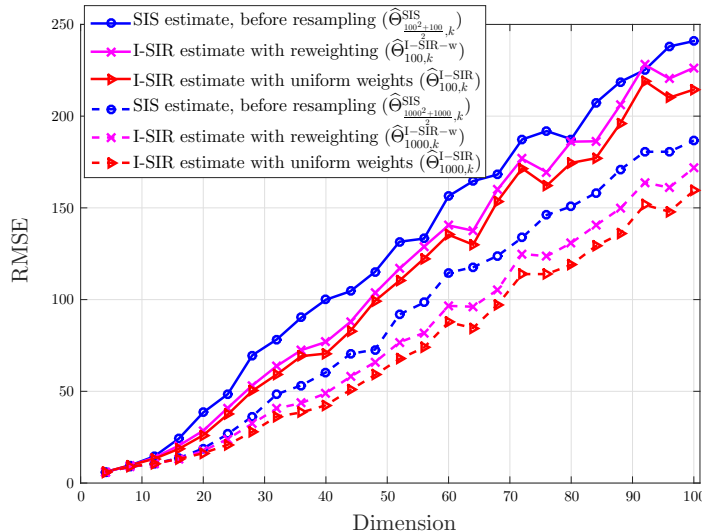
Fig. 4. Multi-dimensional linear Gaussian model - \sigma_Q^2 = 25 , \sigma_x^2 = 4 and \sigma_y^2 = 4 . The estimates of interest are compared as a function of the dimension m of the hidden state x_k for a fixed number of sampling operations. The independent resampling mechanism limits the impact of the large dimension m and estimate \hat{\Theta}_{1000,k}^{I-SIR} when m = 46 has the same performance as \hat{\Theta}_{500500,k}^{I-SIR} when m = 32 .
