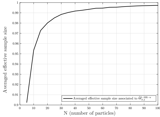
(b) Averaged normalized effective sample size
