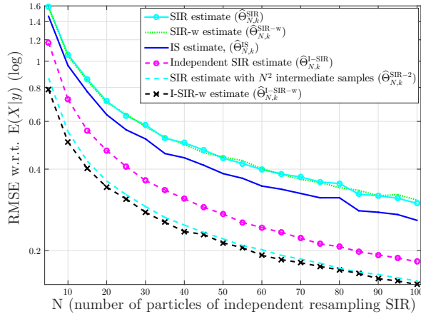
Fig. 1. Static linear and Gaussian model - \sigma_x^2 = 10 , \sigma_y^2 = 3 - Bayesian estimates of E(X|y) based on the independent resampling mechanism outperform the estimates based on the traditional IS and SIR mechanisms although they require an extra computational cost. When the computational cost is fixed, the estimate based on weighted i.i.d. samples from \tilde{q}_N outperforms the estimates based on identically distributed samples from \tilde{q}_{N^2} .
