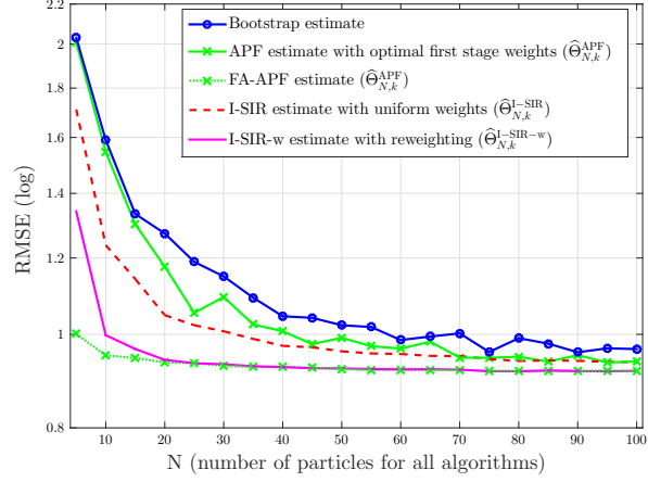
(a) RMSE
