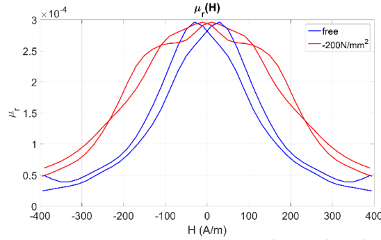
Fig. 1 – Evolution of the RMS permeability versus the excitation field H for a free sample and a stressed one.
