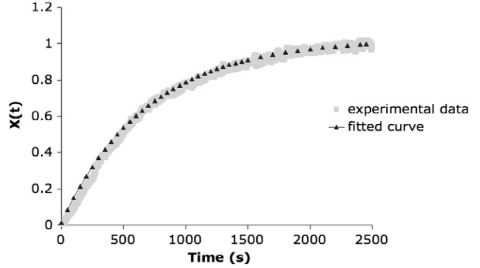
Fig. 8. Correlation between raw data and the fit (2% Silica concentration).
