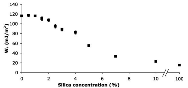
Figure 8. Work of adhesion W_a as a function of the silica concentration.
