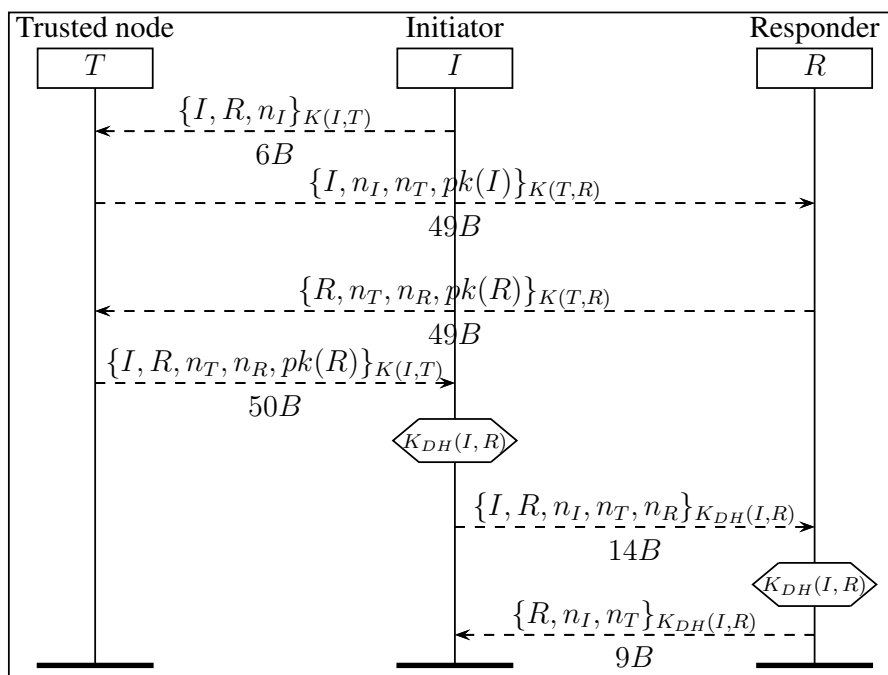
Figure 6. MKE_T - c : Multi-hop Key Establishment using a trusted node T to deliver public keys. T possesses pk(I) but not pk(R) . K_{DH}(I, R) is computed by the initiator I and the responder R .
