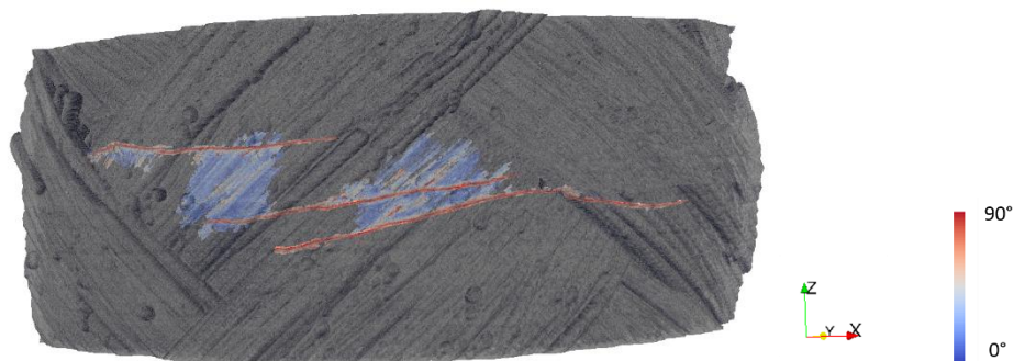
Figure 1: Detected cracks at 204 MPa in a part of the tube (height: 1.5 mm) colored according to the local orientation angles and superimposed to the surrounding microstructure.
