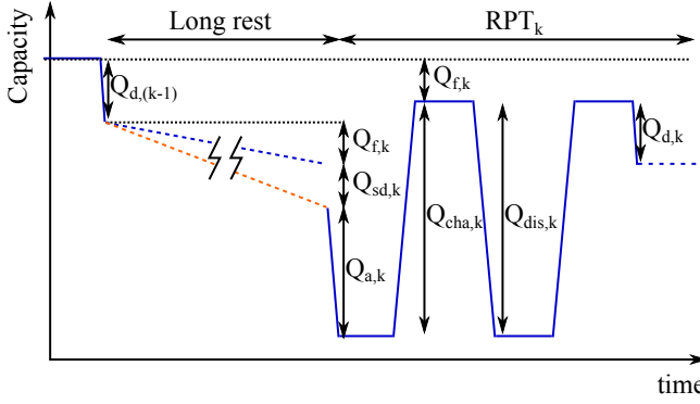
Figure 2: Capacity losses after long rest periods during the k^{th} RPT.
