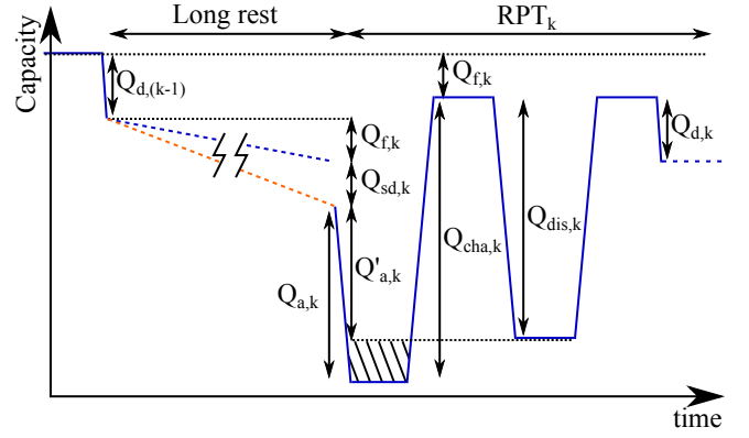
Figure 5: Indirect available capacity measure ( Q'_a ).
