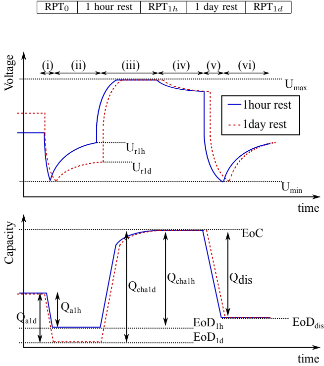
Figure 4: Relaxation effect on Q_a measurement.
