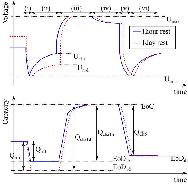
Figure 4: Relaxation effect on Q_a measurement.
