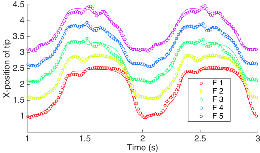
Figure 6 : Tip positions of flap in x-direction within three flow cycles. —: numerical results from LBM : - - -: numerical results from N-S solver, \circ \circ : experiment. The letters F_i indicate the flexible flap number i .
