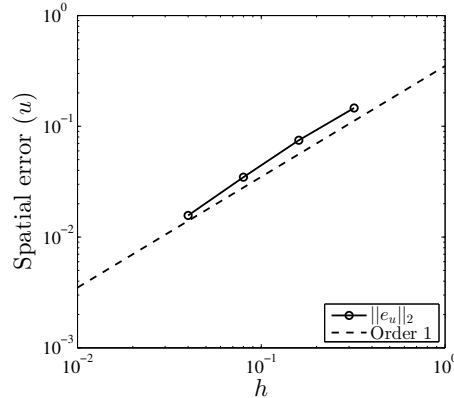
Figure 29. L_2 norm of the horizontal velocity component ( u ) versus grid spacing for the oscillating cylinder problem.
