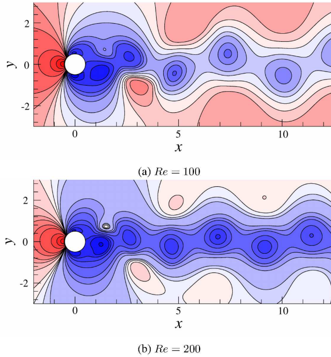
Figure 19. Instantaneous pressure contours of flow over a circular cylinder at (a) Re = 100 and (b) Re = 200 .
