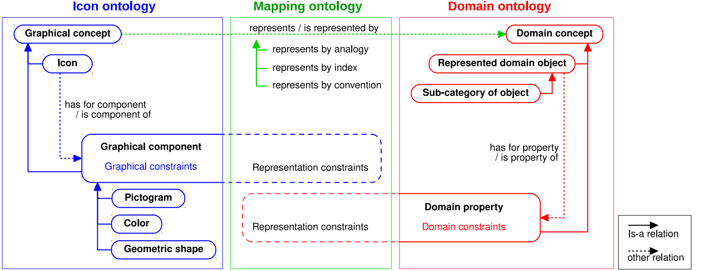
Figure 2: General structure of the icon ontology (in blue on the left), the mapping ontology (in green in the middle) and the domain ontology (in red on the right).
