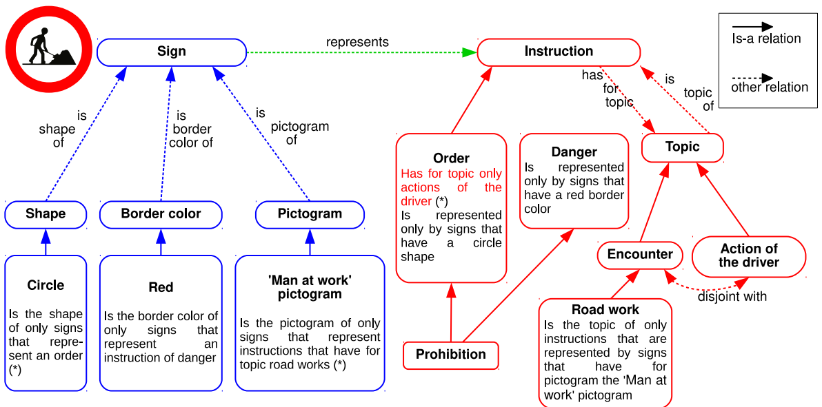
Figure 6: Representation of the inconsistent sign “prohibition of road works” in the traffic sign ontology and the associated semantics. The three constraints marked by a star (*) are the ones that allow inferring the inconsistency of the sign. Two representation constraints allow deducing that this sign represents an order dealing with road works. However, a domain constraint states that orders can be applied only to actions of the driver, and not to encounters such as road work.
