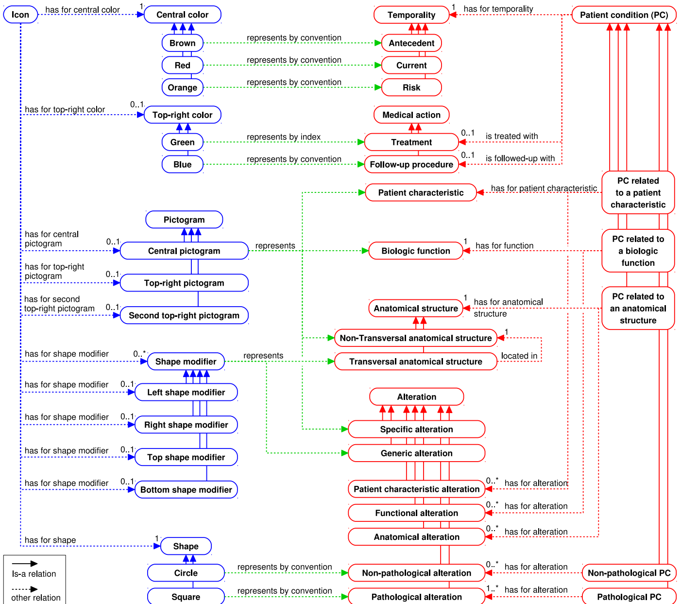
Figure 11: The main concepts and relations in the VCM ontology. The icon ontology is in blue, the domain ontology in red and the “represents” relations in green.
