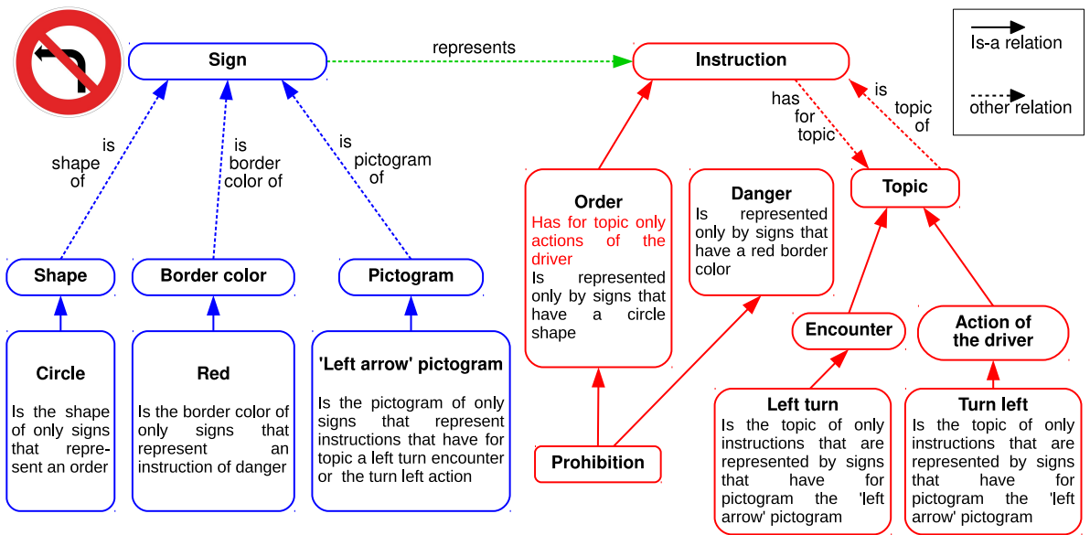
Figure 5: Representation of “prohibition to turn left” in the traffic sign ontology and the associated semantics.
