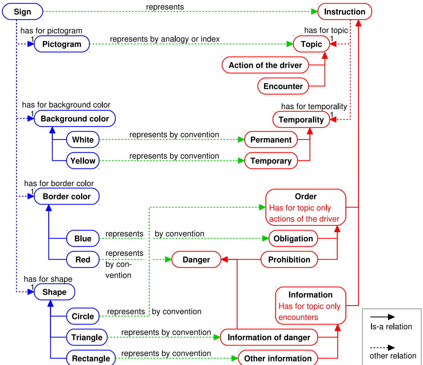
Figure 4: Icon ontology for traffic signs (in blue on the left) and the associated domain ontology (in red on the right).
