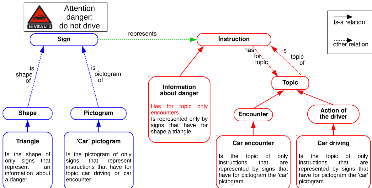
Figure 8: The “pay attention danger: do not drive” icon that figures on some French drug boxes and its representation in the traffic sign ontology. This representation leads to a different meaning for the icon: “pay attention: risk of encountering cars”, because the triangle shape is normally associated with information of an upcoming dangerous encounter, but not with a prohibition.
