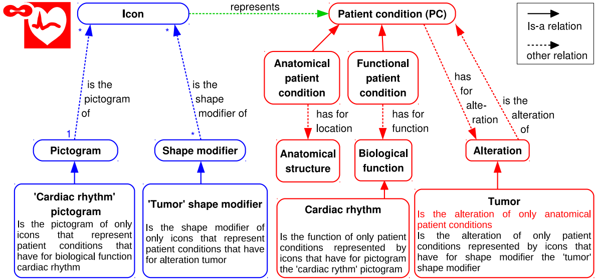
Figure 13: Representation of the “tumor of cardiac rhythm” inconsistent icon in the ontology.
