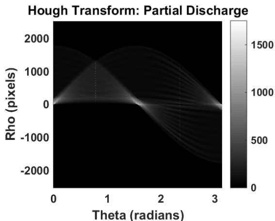
Figure 9. Hough transform of the partial discharge.
