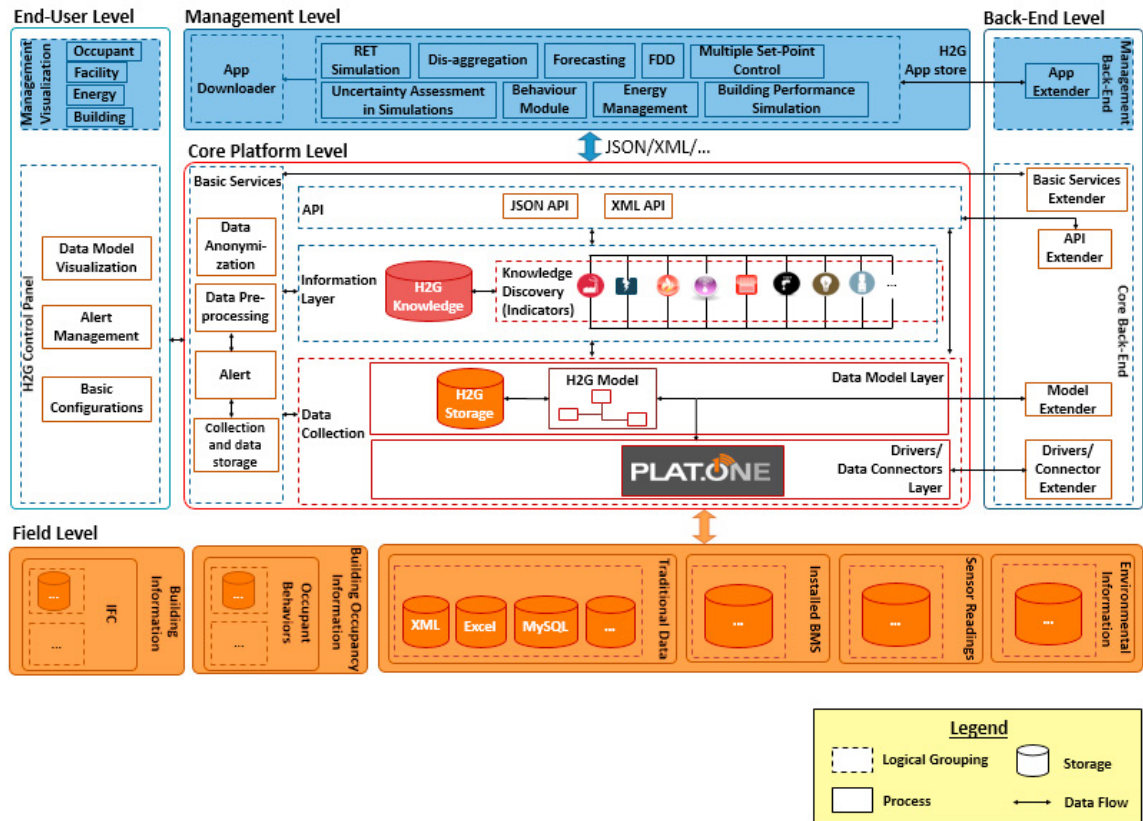
Fig. 1. HIT2GAP Architecture
