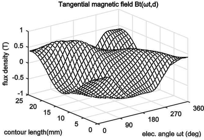
Fig. 3. Tangential magnetic flux density B_t(\omega t, d) along the boundary contour for one electrical cycle for an outer layer coil of the air-core stator.
