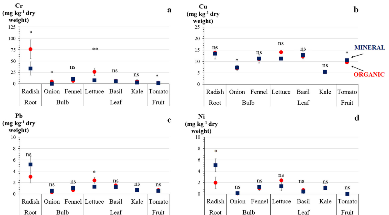
Fig. 3 Accumulation of Cr (a), Cu (b), Pb (c) and Ni (d) (expressed in \text{mg kg}^{-1} dry weight) in edible portions of radish, onion, fennel, lettuce, basil, kale and tomato according to fertilization management (organic in red and mineral in blue). Vertical bars represent standard deviation.
