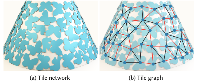
Fig. 11. Tile network and its corresponding graph. Note that (b) only shows the graph for the tiles that are visible in (a). The red edges in (b) form a spanning tree of the graph.
