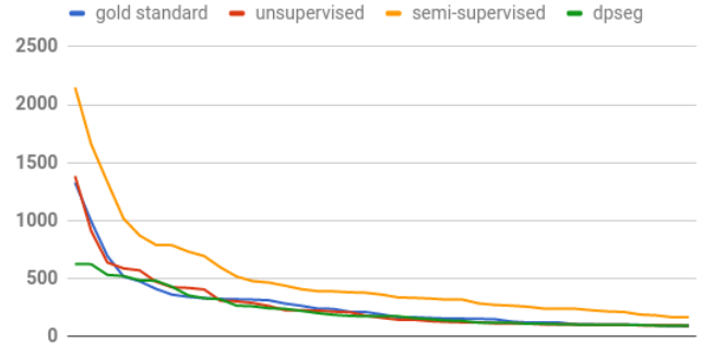
Fig. 2: Word frequency distribution of the three models and the gold standard distribution.
