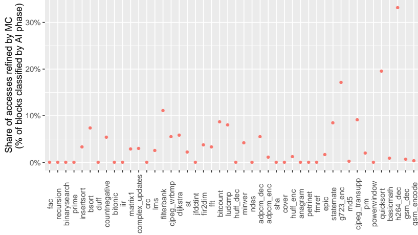
Fig. 6. Increase in hit/miss classifications due to MC relative to pure AI-based analysis.
