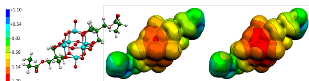
Figure 2. Experimental EP on the molecular surface ( 0.007 \text{ e.Å}^{-3} ) a) structure b) strategy 1 c) strategy 2.
