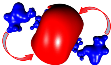
Figure 3. Experimental EP at isovalue surface ( \pm 0.01 \text{ e.Å}^{-1} ) (strategy 2).
