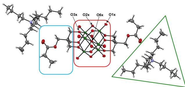
Figure 1. Structure of V6-C3. The red square concerns the V6 core while the blue square concerns the organic moiety. The green triangle indicates the tetrabutylammonium (TBA) counter cation. See Supplementary information for the detail structure description.
