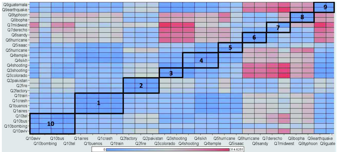
Fig. 4: Cross-temporal analysis of the TREC 2013 TS query-terms.
