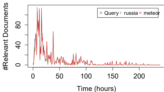
Fig. 8: Time-series of query Q21 and its within terms in the true relevant documents of the TREC 2014 TS track.
