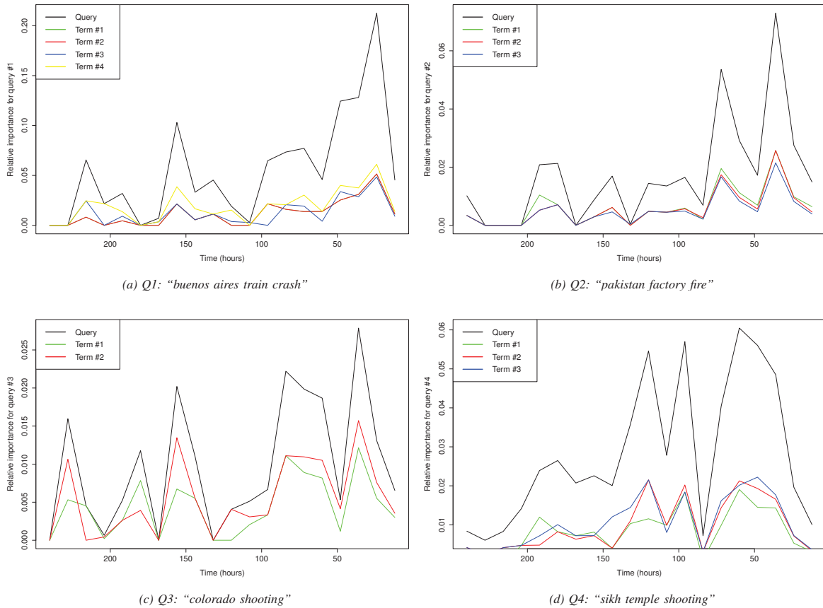
Fig. 2: Time-series analysis of queries Q1-Q4 and their within terms in the true relevant documents (qrels) in the TREC 2013 Temporal Summarization track.
