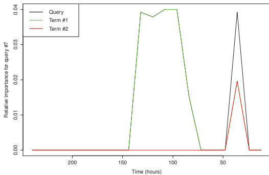
Fig. 5: Distribution over time (measured by hours) of query Q7 (“midwest derecho”) and its within terms in the true relevant documents the TREC 2013 TS track. The x -axis represents time in hours and the y -axis indicates the normalized weight of the query (and terms) over the documents.
