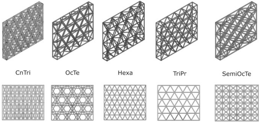
Fig. 2. Grid topologies
