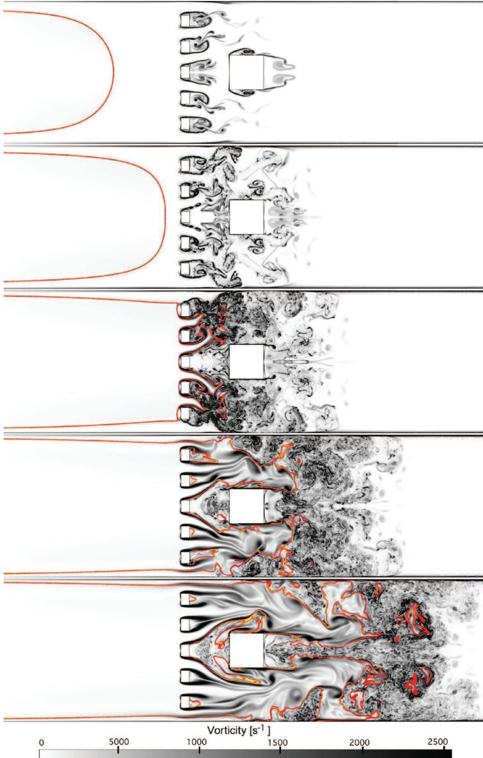
Fig. 18. VRLES ( 973 \cdot 10^6 cells, \Delta_x = 0.136 mm) of flame propagation in configuration OOBSS SS ( C_3H_8 , \Phi = 1 ). Time sequence at t - \Delta t_{peak} = 9.3, 10.8, 11.9, 12.8 and 13.5 ms (from top to bottom). Vorticity field and isoline of heat release.
