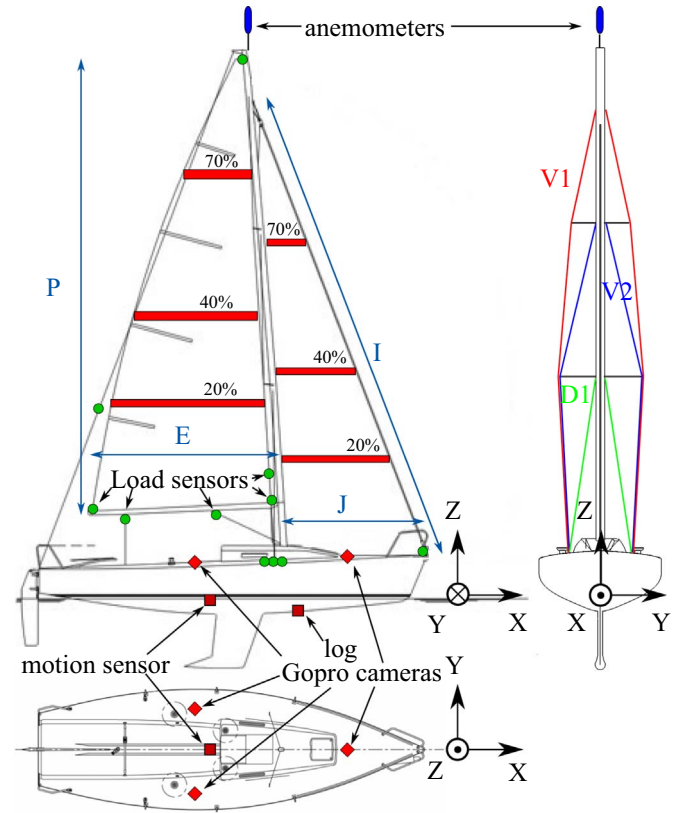
Fig. 1. Yacht system apparatus.
