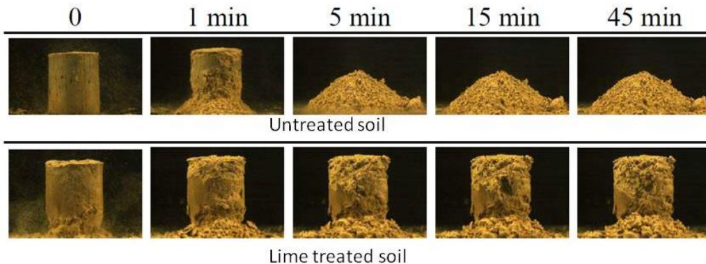
Figure 13. Representative tests results for cores sampled in the treated dike (down), and untreated (above) after 28 days of curing. No evolution observed beyond 45 minutes.
