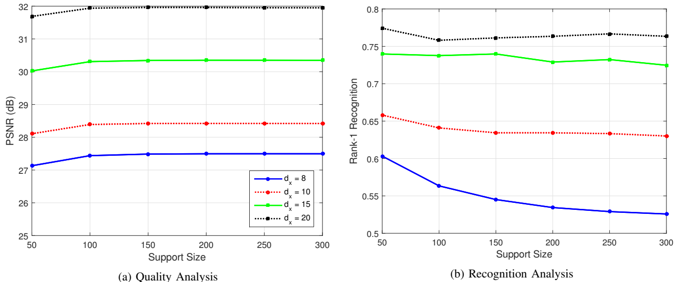
Fig. 9: Analysing the effect of the number of support vectors on the performance of the proposed LM-CSS hallucination method on the FRGC dataset.
