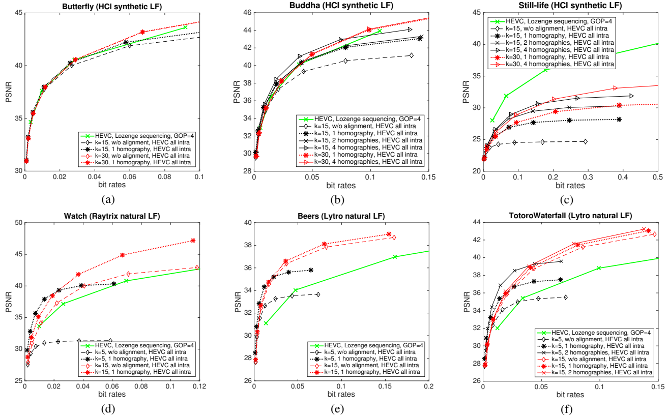
Fig. 2: PSNR-rate performance without and with view alignment for synthetic light fields (Fig. 2a - 2c) or for real light fields (Fig. 2d - 2f) compared with direct HEVC inter coding (green curves).
