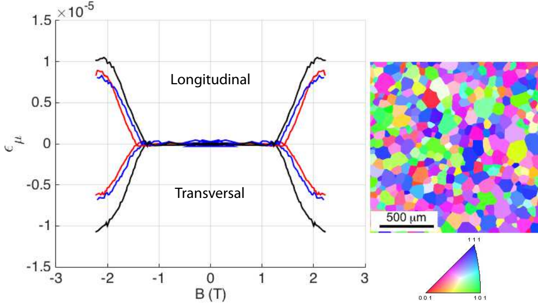
FIG. 1. Magnetostrictive behavior of Fe-27%Co with crystallographic map associated (IPF - ND) for a sample annealed in ferritic phase (red curve along RD, blue curve along 45^\circ /RD, black curve along TD).
