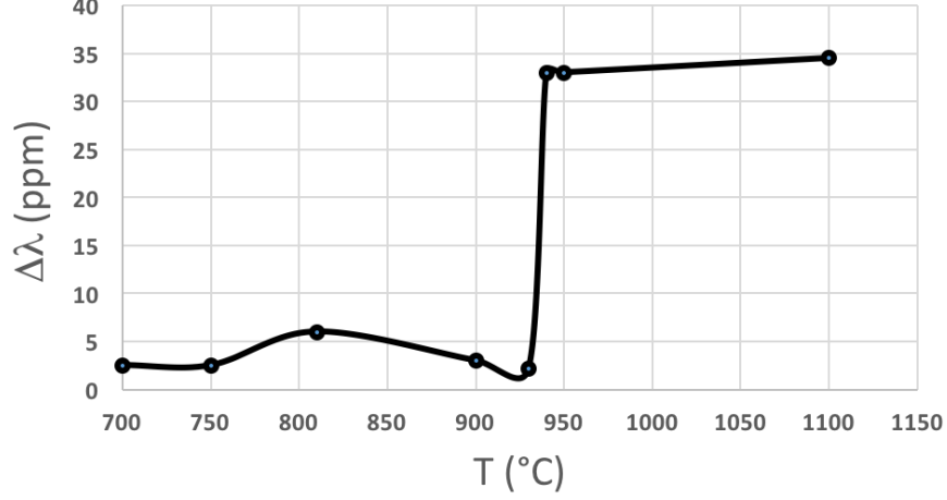
FIG. 3. Evolution of \Delta\lambda at B=1.5\text{T} in terms of annealing temperature.
