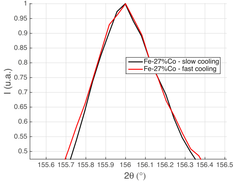
FIG. 7. Compared position of X-Ray diffraction peaks of \{211\} planes for fast (red curve) or slow (black curve) cooling after final annealing at T_3=900^\circ\text{C} -1h-pure \text{H}_2 .
