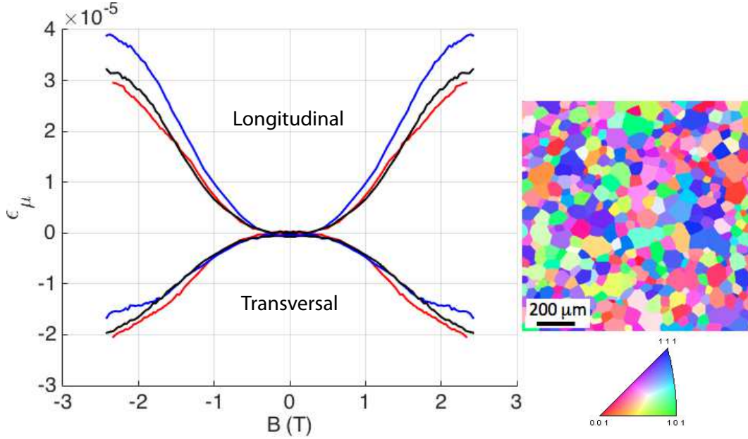
FIG. 2. Magnetostrictive behavior of Fe-27%Co with crystallographic map associated (IPF - ND) for a sample annealed in austenitic phase (red curve along RD, blue curve along 45^\circ/\text{RD} , black curve along TD).
