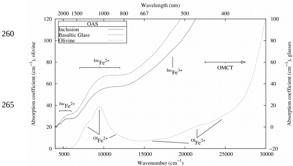
Fig. 3: \mu -Optical absorption spectra of glass inclusions Inc 1, of the surrounding olivine crystal and basaltic glass.
