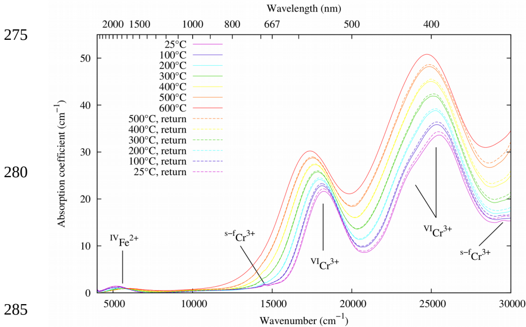
Fig. 4: \mu -Optical absorption spectra measured between room temperature and 600^\circ\text{C} on a natural spinel crystal ( \text{MgAl}_2\text{O}_4 ) containing \text{Fe}^{2+} and \text{Cr}^{3+} impurities. The crystal is 0.5 \text{ mm} thick. The spectra denoted “return” are recorded during cooling, after heating at 600^\circ\text{C} . The coordination of the cation at the origin of each band is indicated, s-f stands for spin-forbidden transition.
