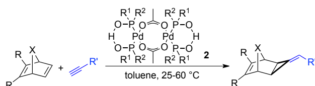
Scheme 2. Hydroalkynylation versus [2+1] cycloaddition: chemodivergent palladium-promoted transformations
