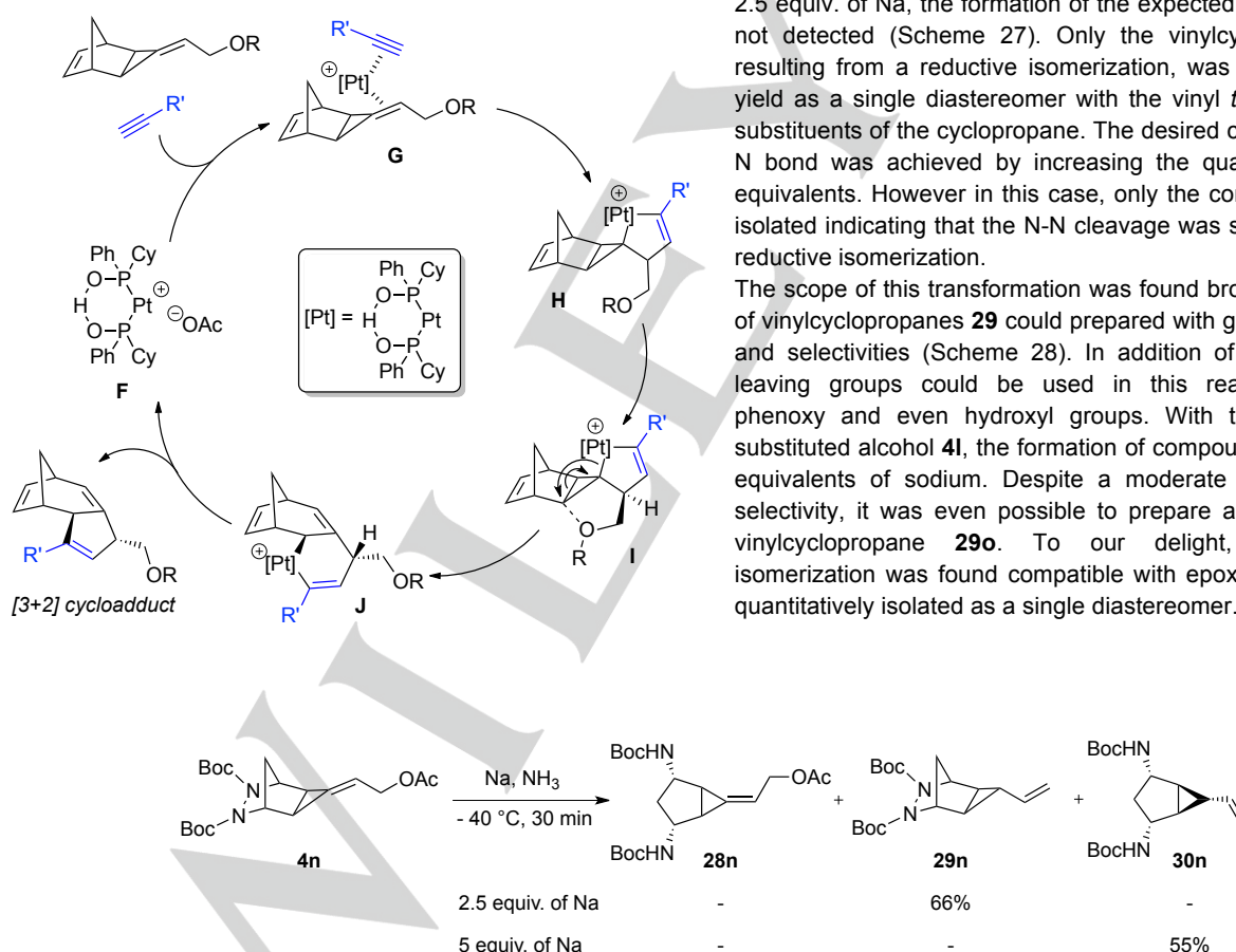
Scheme 27. Reductive cleavage of the nitrogen-nitrogen bond of cyclic hydrazine 4n .
