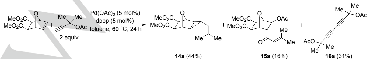
Scheme 16. Control experiments using 1,3-bis(diphenylphosphino)propane (dppp) as ligand.
