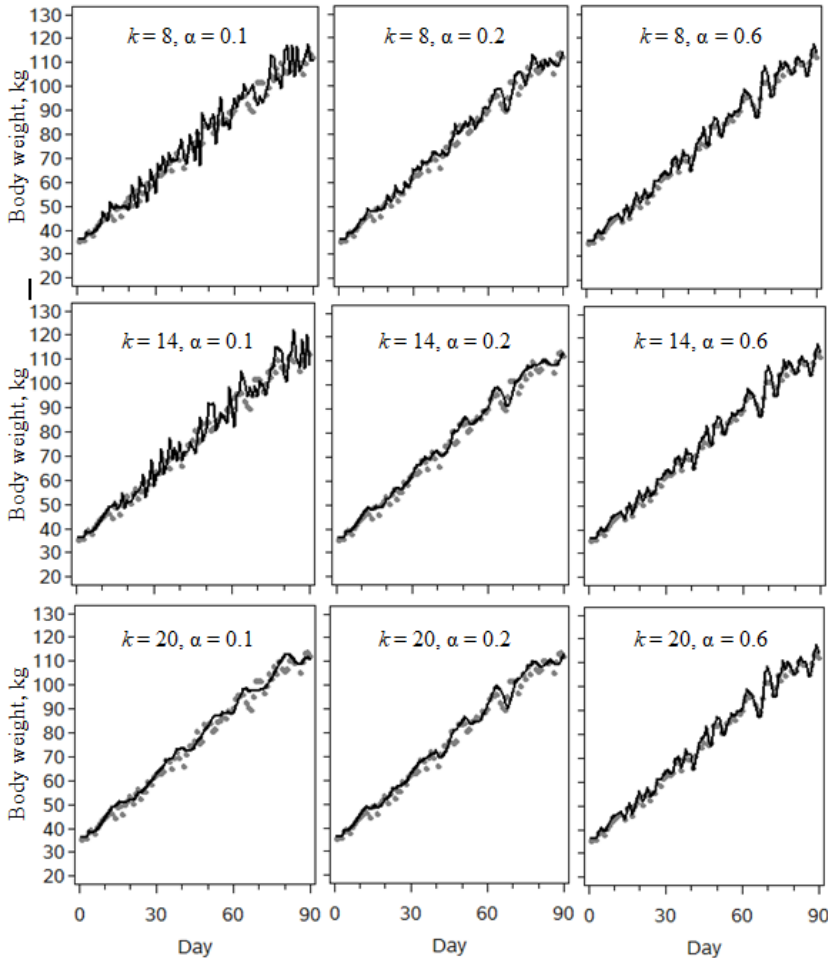
Figure 1 part 1: Example of comparison of measured (●) to forecasted (—) BW with the HW method implemented with the 8, 14 or 20 latest values ( k ) and three values for the smoothing parameter \alpha (fig 310 in trial 1). To be continued...
