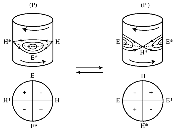
FIG. 6. (Bottom) Sketch of vertical velocity variations in the equatorial plane of the pure modes P and P' . The (+) sign designates upward and (-) sign designates downward vertical velocities. The heteroclinic cycle connects P and P' , related by rotation of \pi/2 . The radial vortices are centered on the diametrically opposite elliptic points ( E, E^* ) and are located at right angle from the hyperbolic points ( H, H^* ). (Top) Perspective representations of the two corotating vortices separated by the two hyperbolic points ( H, H^* ).
