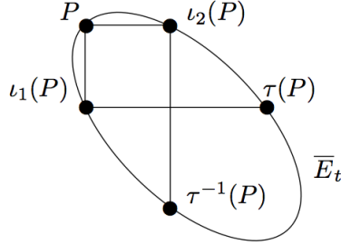
FIGURE 4. The maps \iota_1 and \iota_2 restricted to the kernel curve \overline{E}_t
