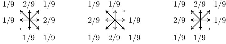
FIGURE 9. Three models with a group of order 10. These models, proposed in [KY15] and conjectured to be algebraic, were recently solved in [BBMR17]
