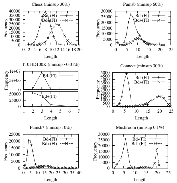
Figure 1. Borders of frequent itemsets
