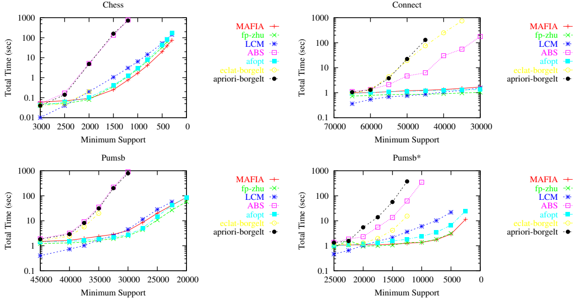
Figure 5. Algorithms performances
