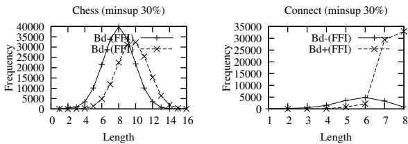
Figure 3. Borders of frequent free itemsets
