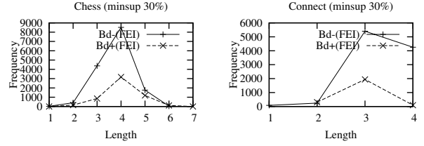
Figure 4. Borders of frequent essential itemsets
