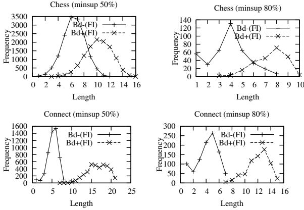
Figure 2. Borders of frequent itemsets with a different minimum support threshold
