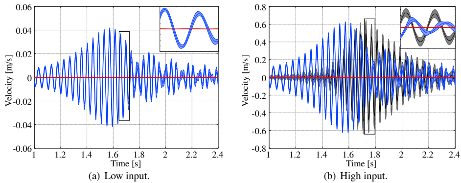
Fig. 5. Confidence bands for the kernels contribution to the output signals obtained through the Volterra model with 99% of confidence. ■ represents the linear contribution, ■ represents the quadratic contribution and ■ represents the cubic contribution.
