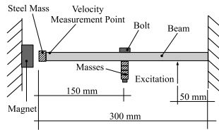
Fig. 2. Experimental setup (scheme) [6].
