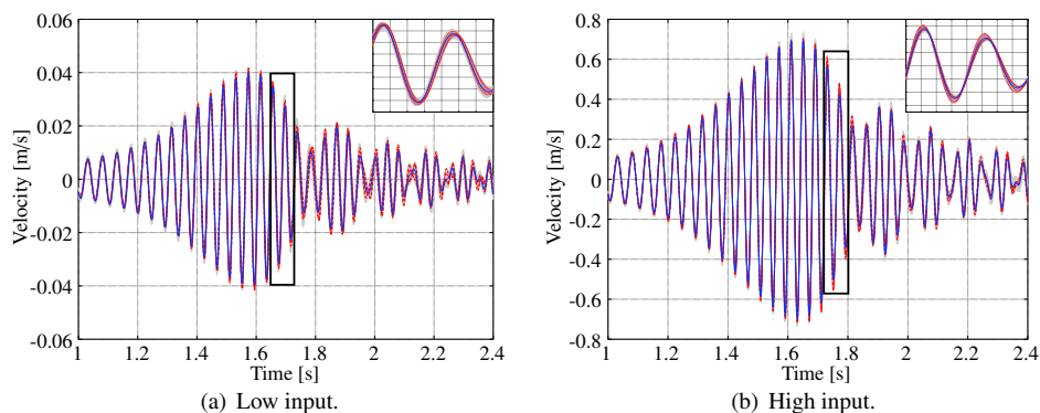
Fig. 4. Confidence bands for the system responses obtained through the Volterra model with 99% of confidence. The mean is represented by the blue line and the experimental data by the red dots.
