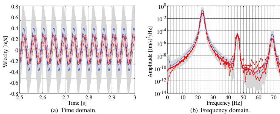
Fig. 6. Confidence bands for the system responses obtained through the Volterra model with 99% of confidence. The mean is represented by the blue line and the experimental data are represented by the red line.
