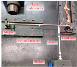
Fig. 1. Experimental setup (photo) [6].
