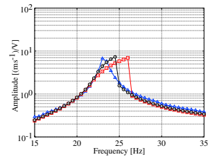
Fig. 3. Beam velocity during a stepped sine test, where \Delta represents the low level of input signal (0.01 V), \circ the medium level (0.10 V) and \square the high level (0.15 V).
